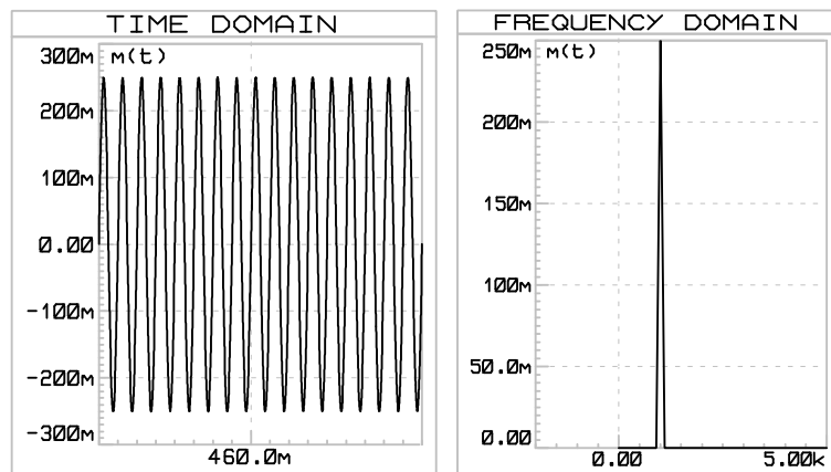
MESSAGE SIGNAL m(t)
