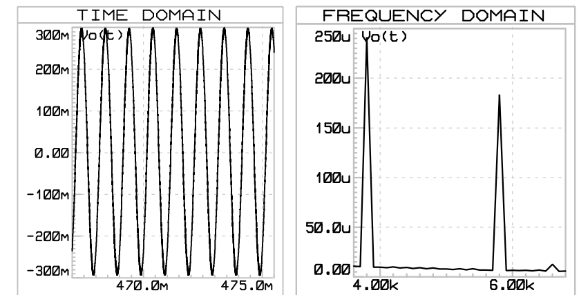
DEMODULATION SIGNAL V_o(t)
